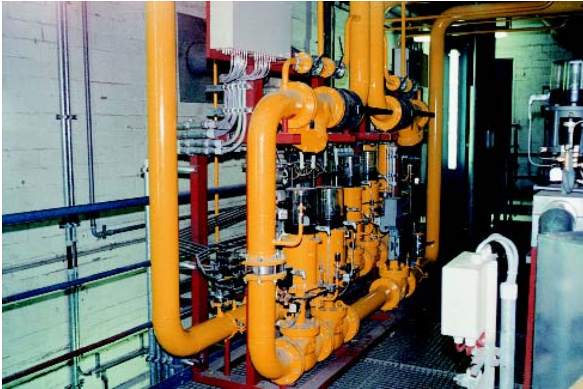
Natural Gas Measuring and Control Station for a gas-fired steam boiler in an industrial power plant
